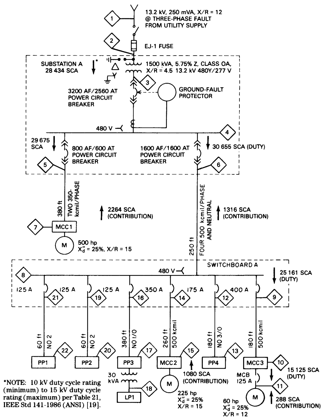
Figure 101—Typical Distribution Single-Line Diagram (Coordination Example)
