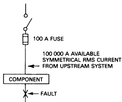
Figure 118—Application Example of Fuse Let-Through Charts
