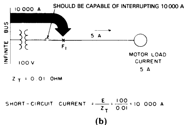
Figure 79—Short Circuit on Load Side of Main Switch
