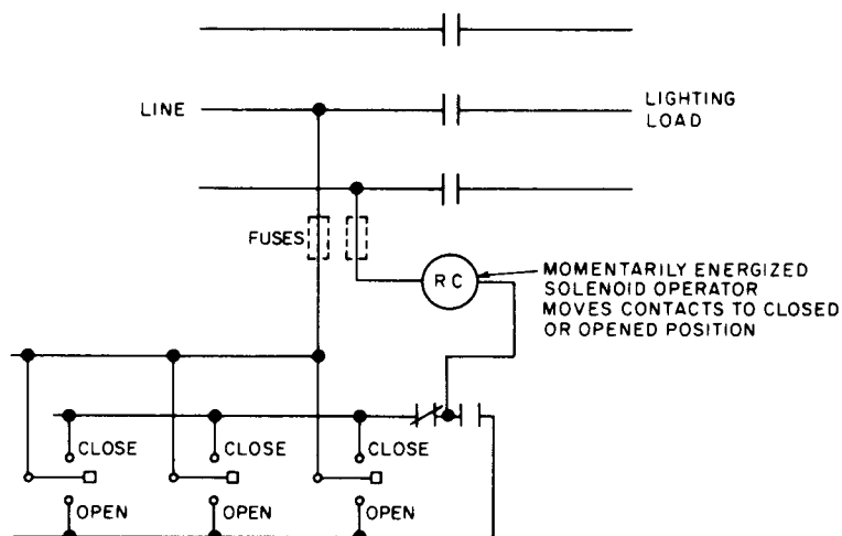
(c) Mechanically Held Electrically Operating Lighting Contactor Controlled by Multiple Momentary-Toggle-Type Control Stations
