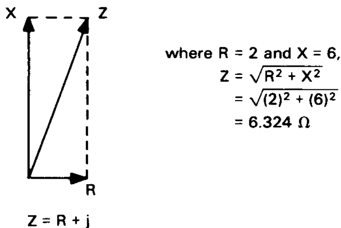
Figure 92—Impedance Vectors
