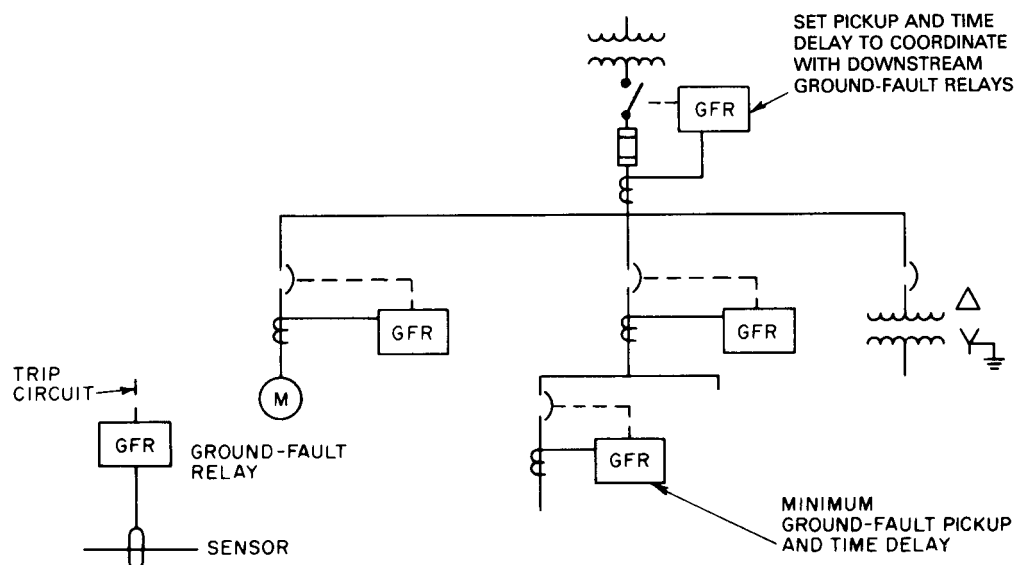
Figure 125—Typical Ground-Fault Relaying
