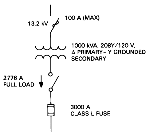
Figure 121—Typical Low-Voltage Distribution Transformer Secondary Protection
