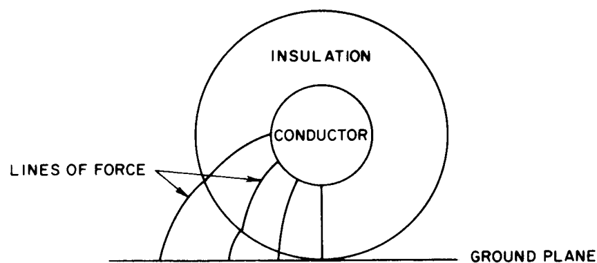
Figure 65—Unshielded Cable on Ground Plane
