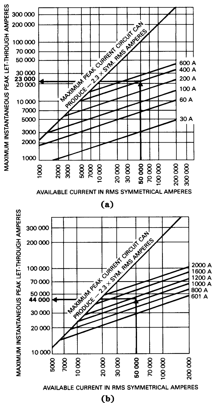
Figure 98—Typical Current-Limiting Fuse Peak Let-Through Curves (a) (Class RK1) Peak Let-Through Current Data at 600 V ac (b) (Class L) Peak Let-Through Current Data at 600 V ac
