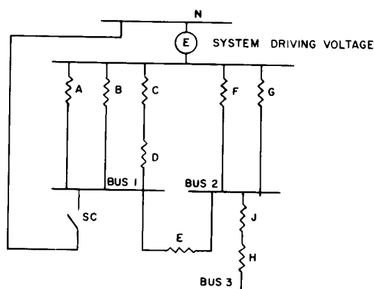
Figure 91—Equivalent Impedance Diagram for System in Fig 90
