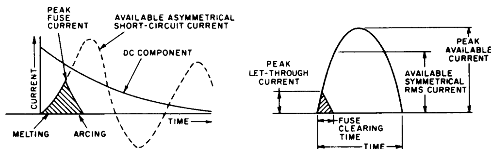
Figure 48—Current-Limiting Action of Fuses
