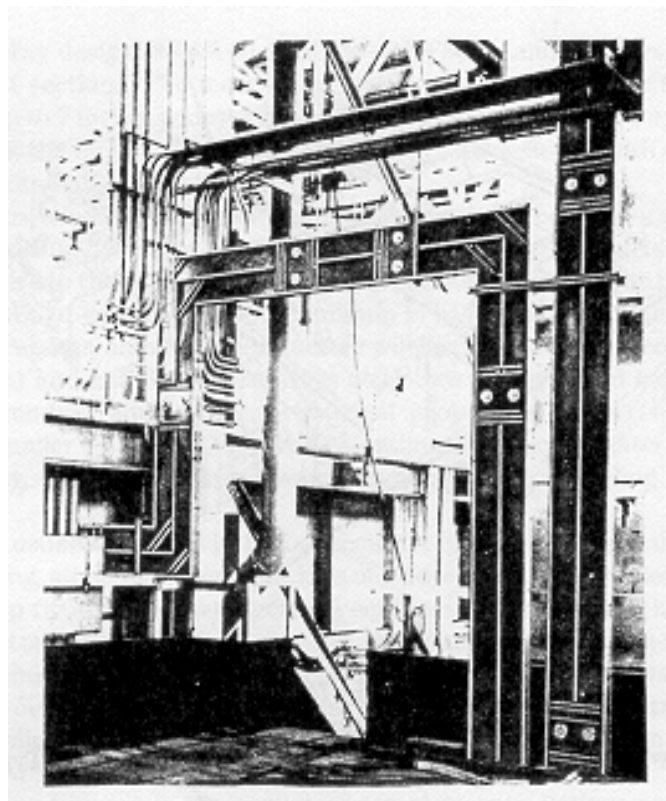
Figure 75—Feeder Busway
