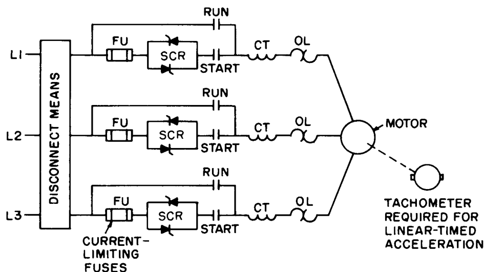
Figure 57—Simplified Wiring Diagram of a Solid-State Controller
